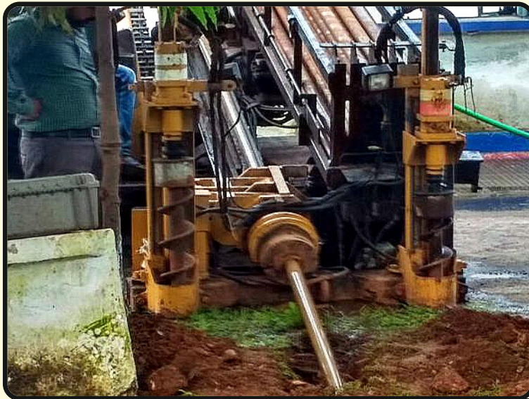
Construction of Optical fiber Laying with HDD for TCIL - Vizag
